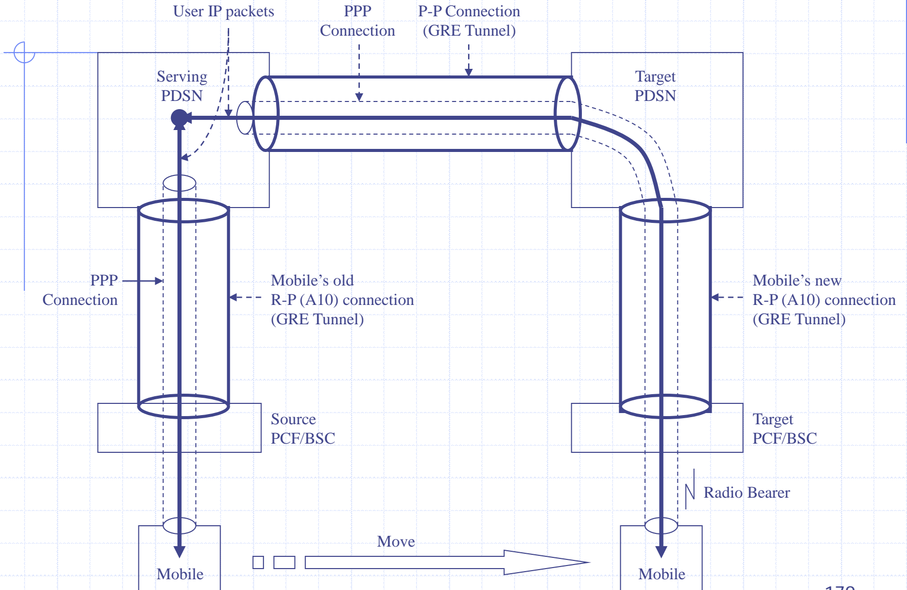
Fig. 4.62 3GPP2 fast inter-PDSN handoff: user traffic flow
