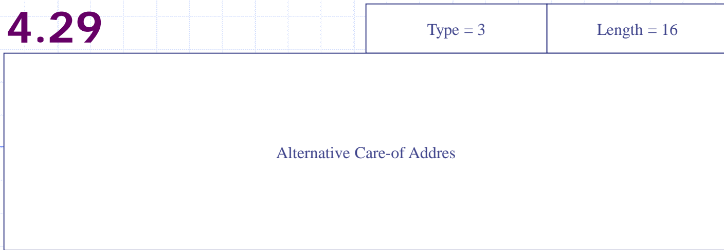
(a) Format of Alternative Care-of Address option.
