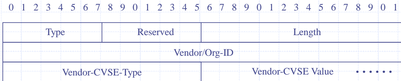
(a) Critical Vendor/Organization Specific Extension (CVSE)
