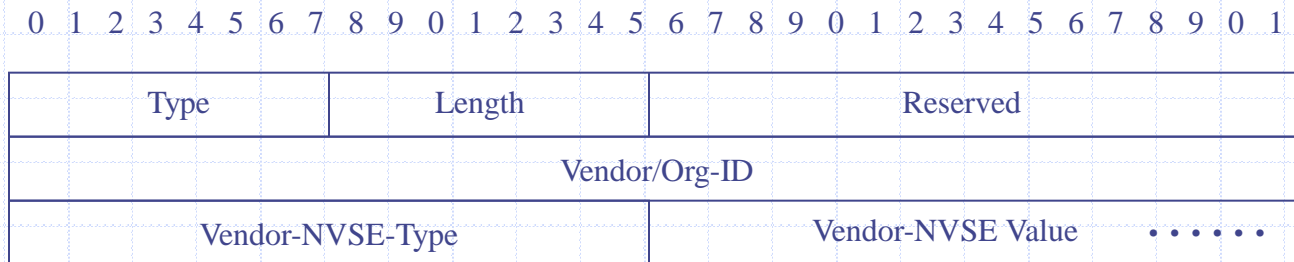
(b) Normal Vendor/Organization Specific Extension (NVSE)
