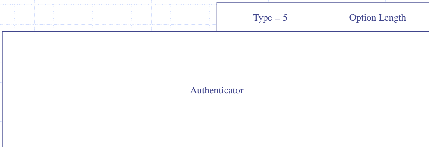
(b) Format of Binding Authorization Data option.
