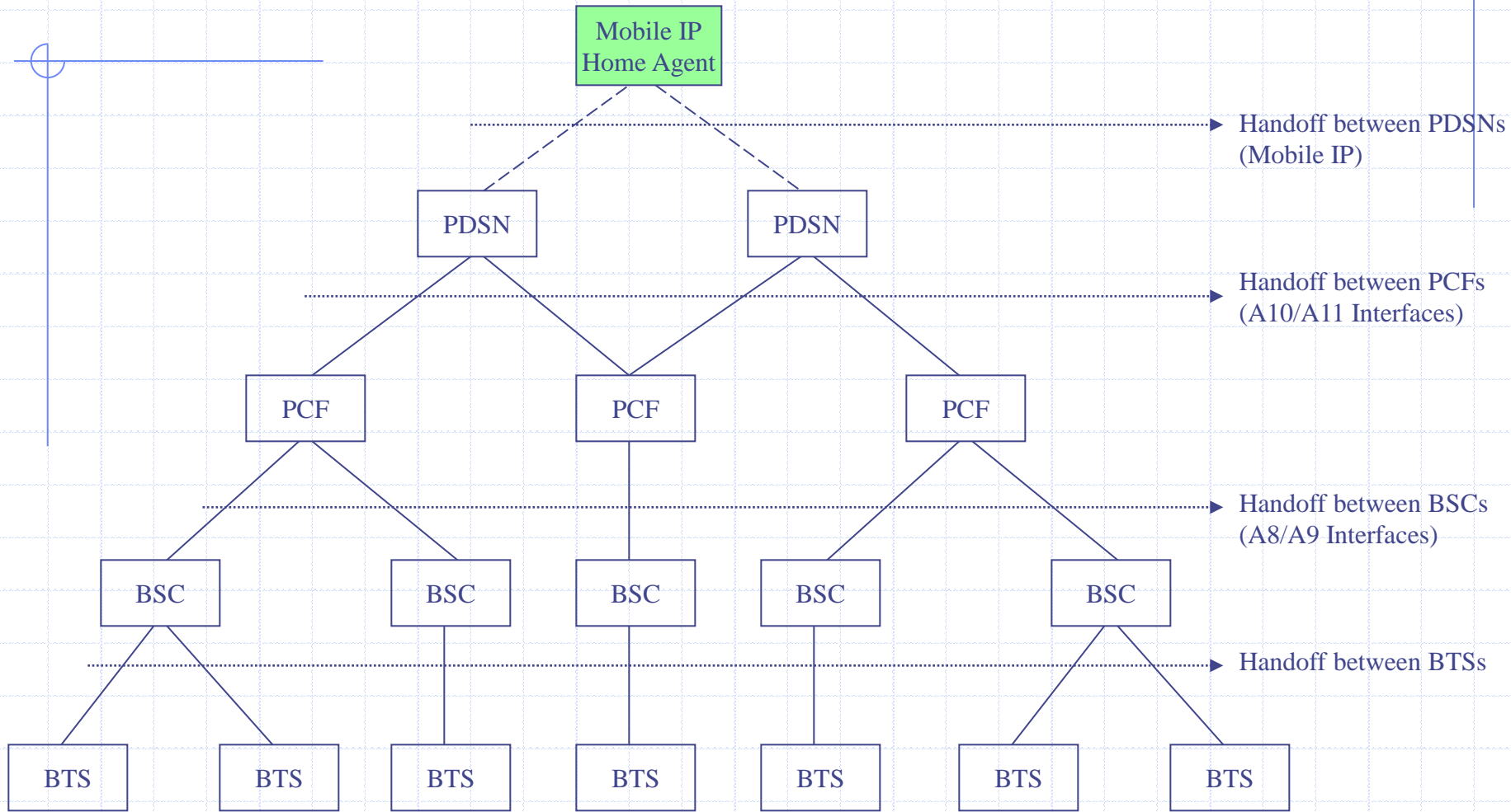
Fig. 5.56 Scopes of mobility in a 3GPP2 packet data network
