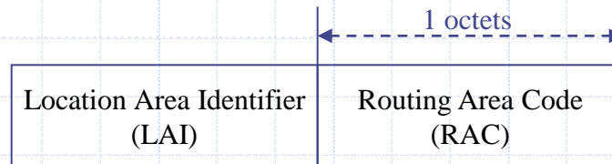
(a) Structure of Routing Area Identifier (RAI)
